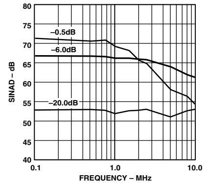
TPC 24. SINAD vs. Input Frequency (Input Span = 5.0 V p-p, V_{CM} = 2.5 \text{ V} )
